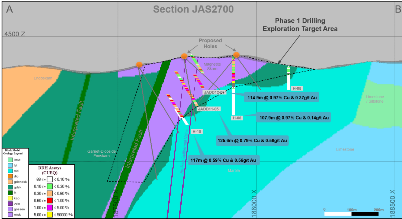
Figure 2: Section line JAS2700, showing historic drilling, significant assays, and geologic interpretation
