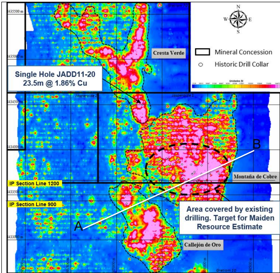
Figure 1: Ground magnetic analytical signal image over the Greatiam 10 & 70 and Jasperoide 1 & 2 Exploration Concessions showing high-priority areas for surface exploration and drilling
