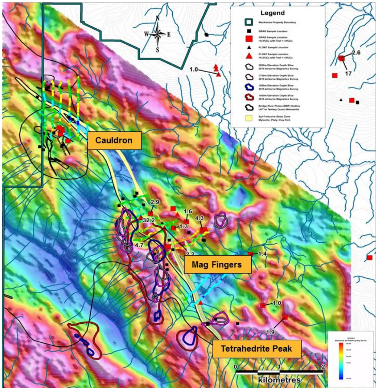
Mackenzie Project Bornite Trend showing 3 copper zones on TMI Magnetics
